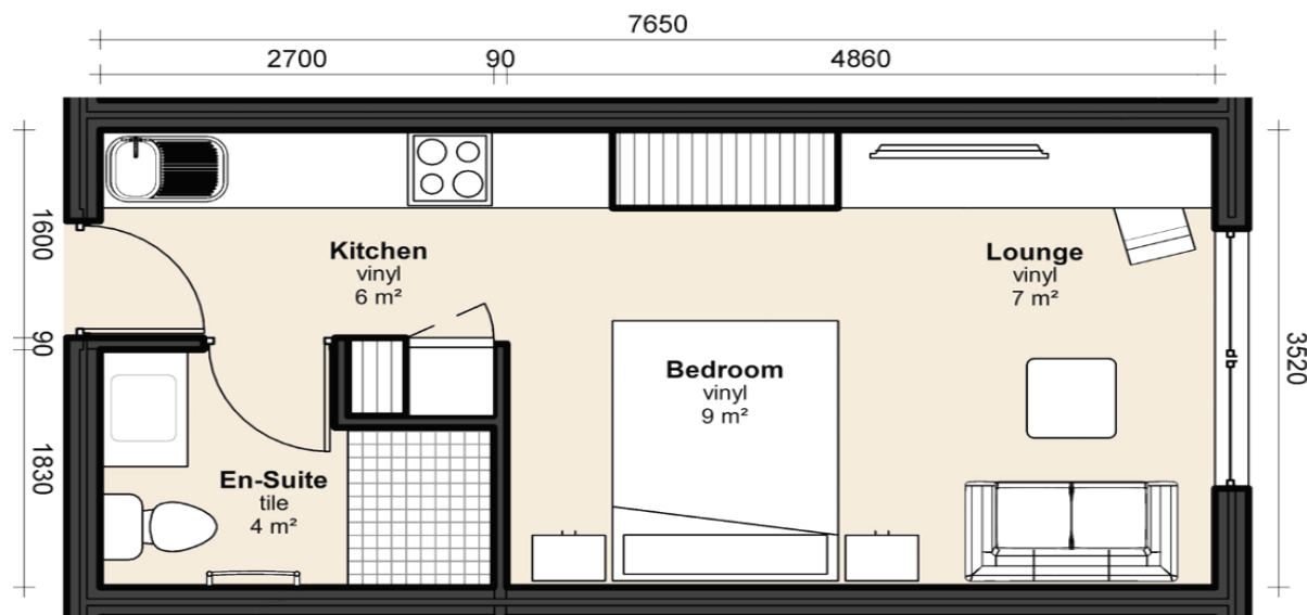
Typical Unit Floor Plan Unit Size 30 sqm
